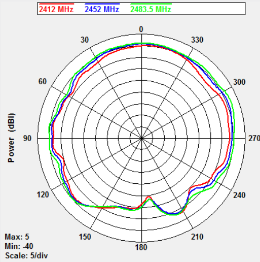
2.4G (PHI=90)
