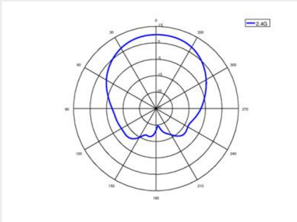
2.4G (PHI=0)
